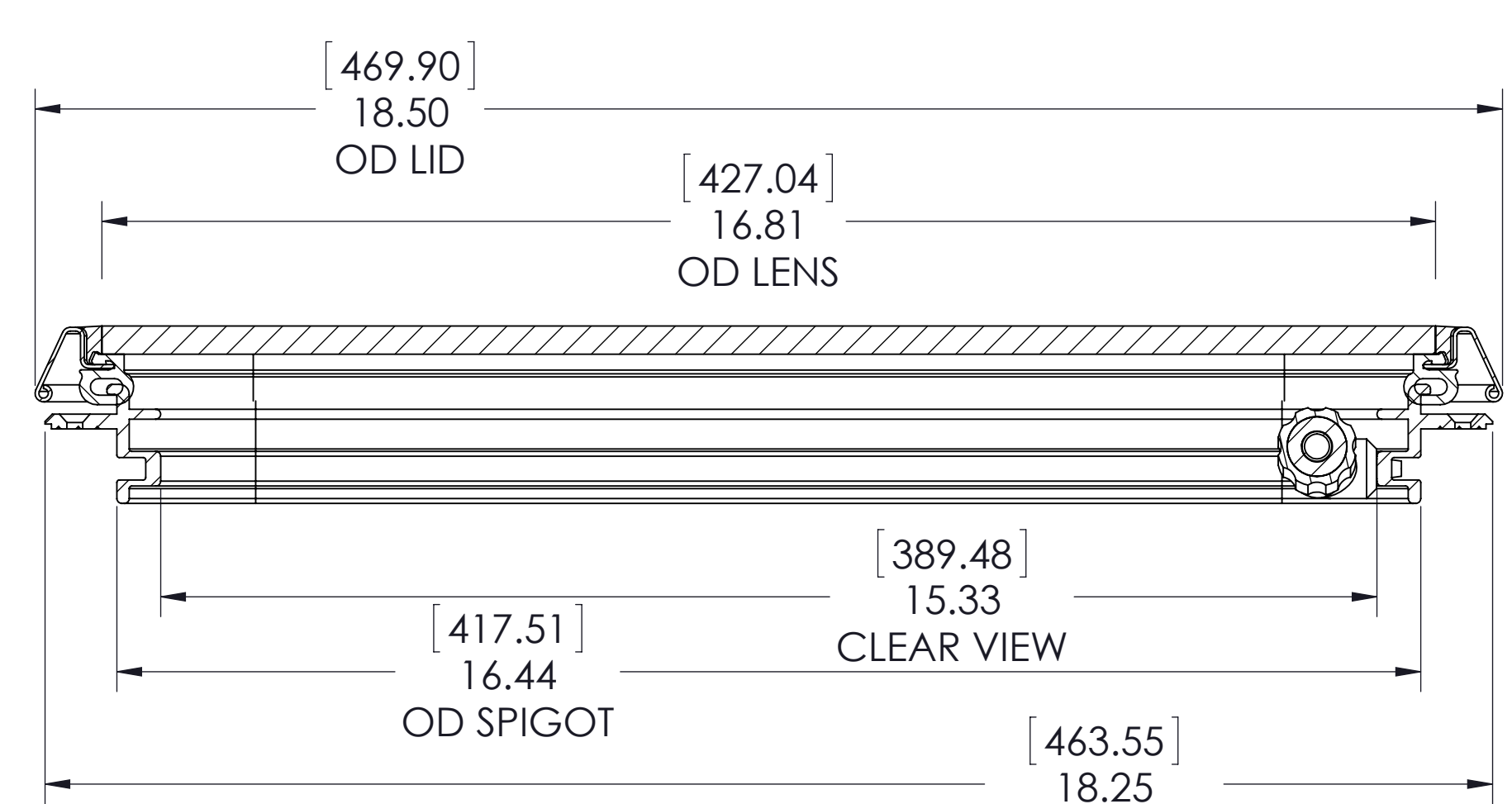
SECTION B-B
