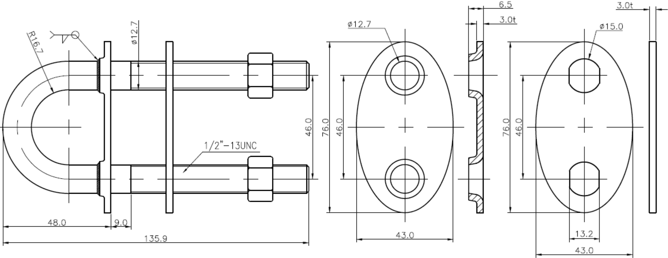
WELDED PLATE
